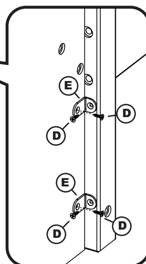
BACK BOTTOM VIEW
