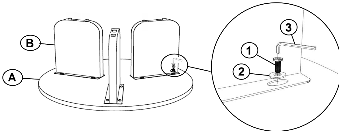
BOTTOM VIEW
