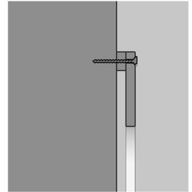
Wall-mounted section
