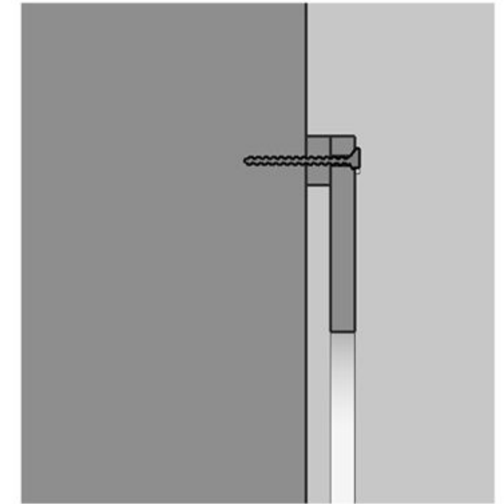
Wall-mounted section
