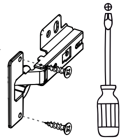
Hinge adjustment
