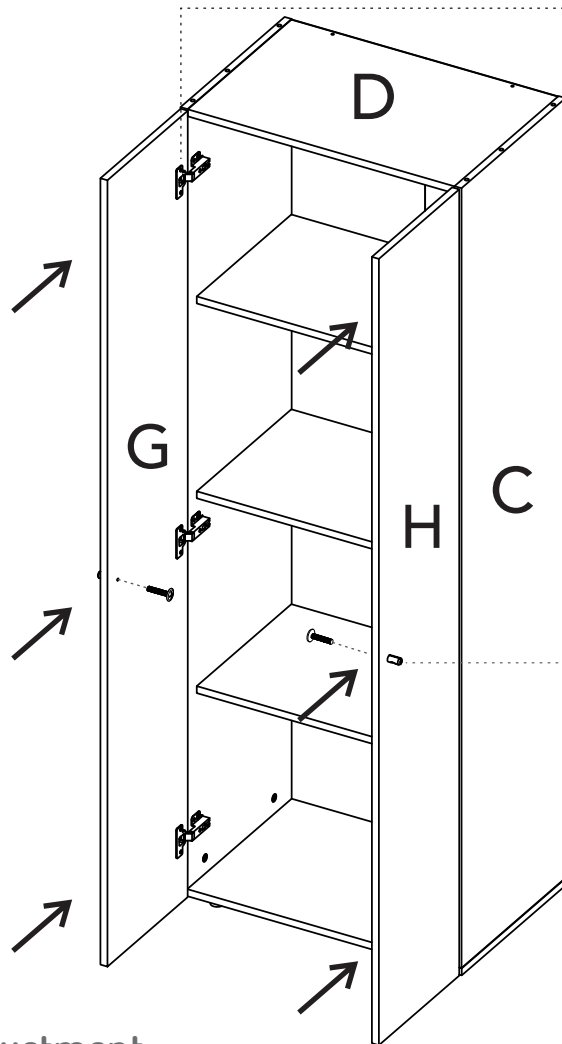
Hinge adjustment
