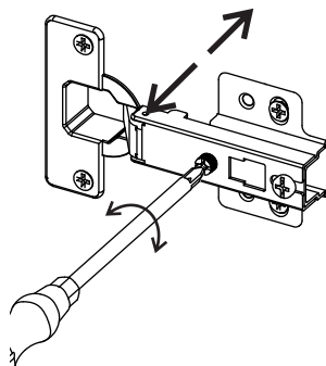
Lateral adjustment
