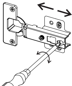
Depth adjustment
