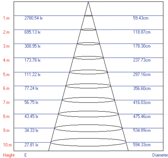
Lux-Distance Curve
