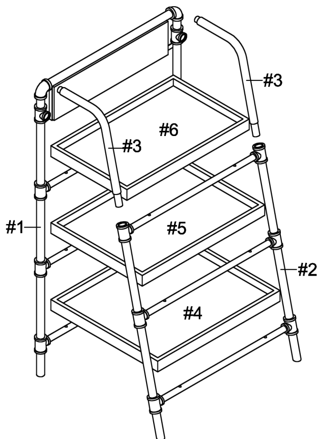
Exploded View
