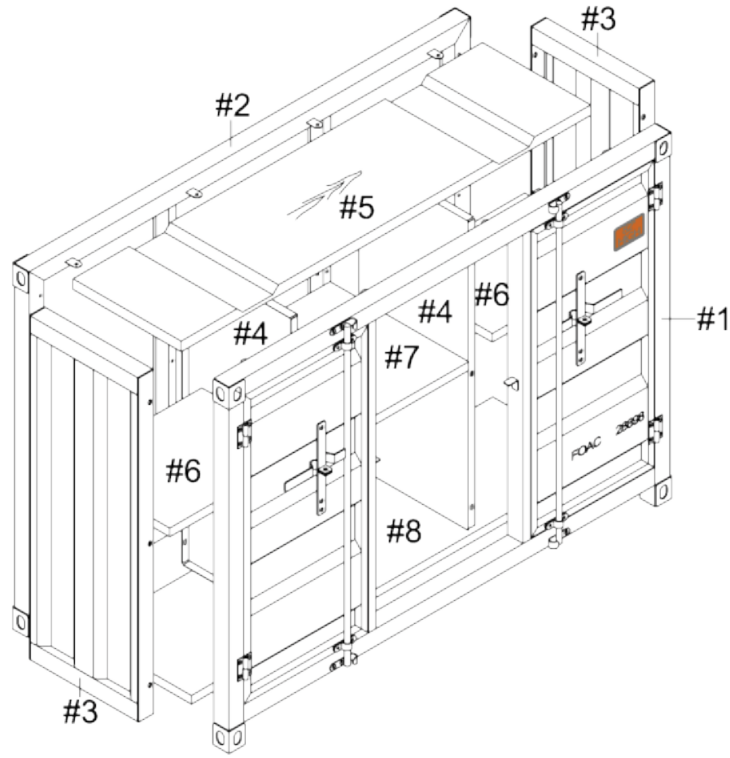
Exploded View
