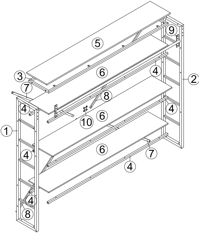
Exploded View
